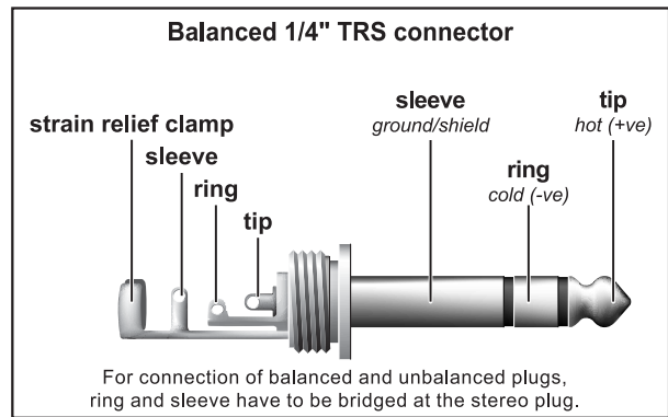
Fig. 4.4: 1/4" TRS connector
